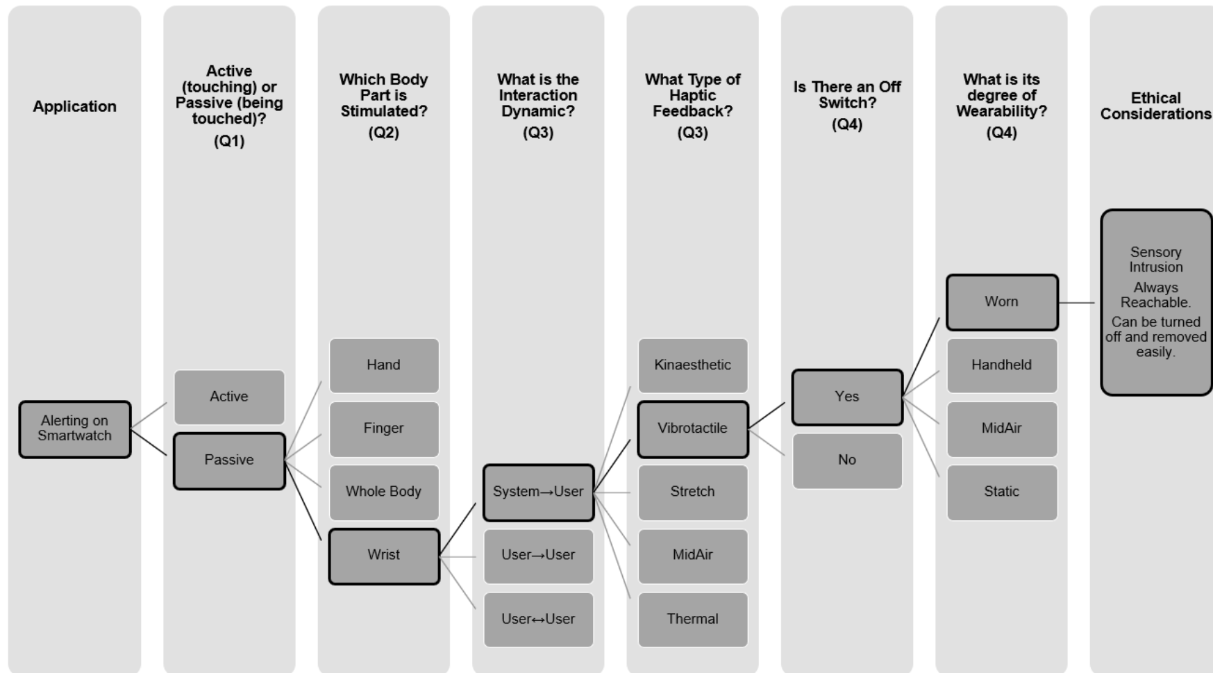
FIGURE 2(b). The four ethical questions used as a decision tree to determine relevant ethical considerations for a hypothetical tactile alerting device. Black outline and black lines indicate the path taken.
