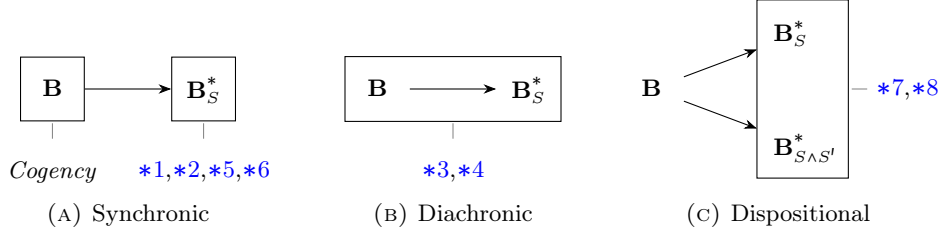
FIGURE 1. The relation of the three types of coherence
