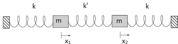
Fig. 1. Coupled masses on springs.
