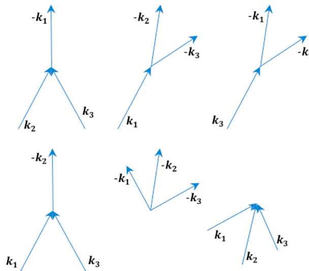
Fig. 3. Diagrams for three phonon processes: for example the top left diagram represents \hat{a}_{-\mathbf{k}_1j_1}^\dagger \hat{a}_{\mathbf{k}_2j_2} \hat{a}_{\mathbf{k}_3j_3} .
