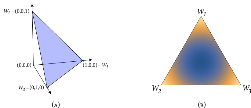
FIGURE 2. In figure 2a: the 2-simplex of probability distributions over three worlds is given by all points lying in the convex hull of W_1 = \langle 0, 0, 1 \rangle , W_2 = \langle 0, 1, 0 \rangle , and W_3 = \langle 1, 0, 0 \rangle . In figure 2b, a ‘heat map’ for the magnitude of these probability distributions. Probabilities closer to individual worlds have greater magnitudes (represented with ‘hotter’ colours), and probabilities further away have small magnitudes (represented with ‘cooler’ colours).
