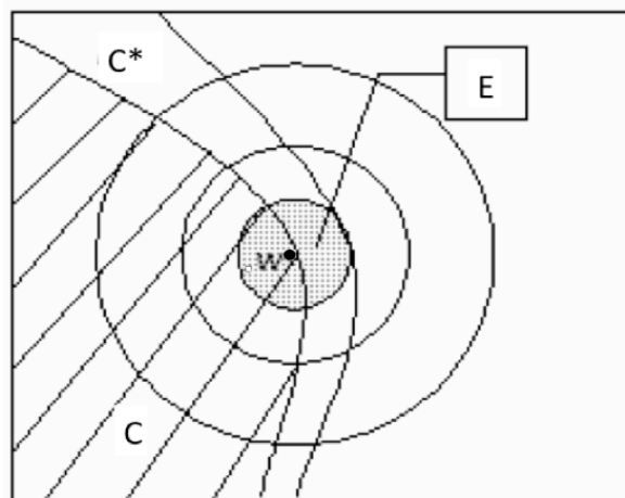
Figure 1: Realization-insensitive causation
