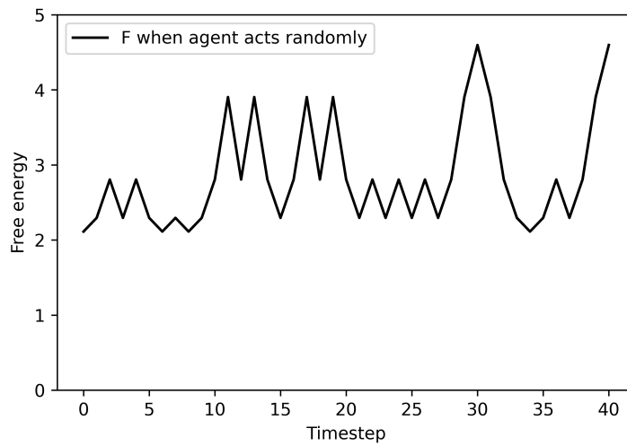
Figure 6: Variational free energy over time for an agent that acts randomly. After 42 timesteps the agent dies. The code to generate this figure can be found at https://github.com/stephenfmann/fep .
