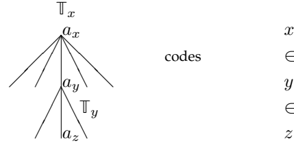
Figure VII.2: An example of a tree corresponding to a coding pair showing membership.
