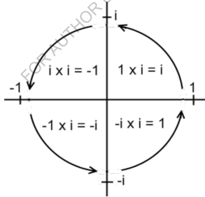
Figure 2 – WICK ROTATION: “The complex plane reveals i 's special relationship with cycles via the circle of i , also known as Wick rotation. Whenever a point on the complex plane is multiplied by i , it moves a quarter rotation around the origin or center of the plane.” [Figure and quote from Welch (2015)]
