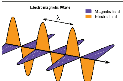
Figure 1 - An electromagnetic wave showing electric and magnetic fields, and the wavelength ( \lambda ) which is the distance between crests of a wave.
