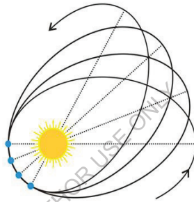
Figure 2 - Mercury's orbit (above) with its perihelion's constant level on the left and ascending pattern on the right
