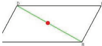
Fig. 4 – VTS (VECTOR-TENSOR-SCALAR) GEOMETRY - Interaction of Gravitation and Electromagnetism Produces a Momentum in Gravitons and Photons (and a Pressure Which is Known as Mass). VTS Geometry inspired by Einstein (1919)
