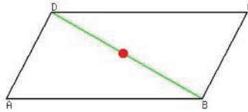
Figure 3: VTS (VECTOR-TENSOR-SCALAR) GEOMETRY - Interaction of Gravitation and Electromagnetism Produces a Momentum in Gravitons and Photons (and a Pressure Which is Known as Mass). VTS Geometry inspired by Einstein(1919)
