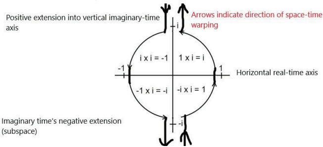
Figure 12 – Spacetime Warping Associated With Imaginary Computer
