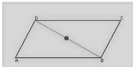
Figure 11: Vector-Tensor-Scalar Geometry
