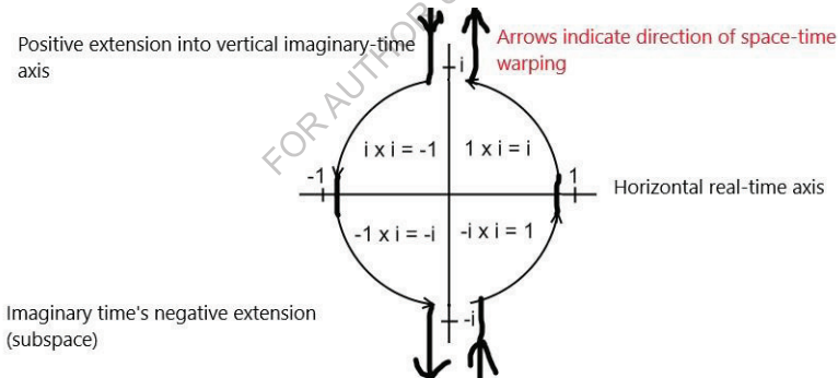
Figure 2: SPACE-TIME WARPING IN IMAGINARY COMPUTER
