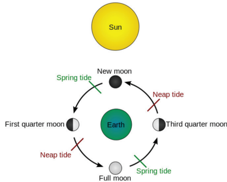
Figure 5 – TIDE SCHEMATIC - Does explanation of spring and neap tides require combining the theories of Newton, Kepler and Galileo? - public domain image from https://en.wikipedia.org/wiki/File:Tide_schematic.svg
