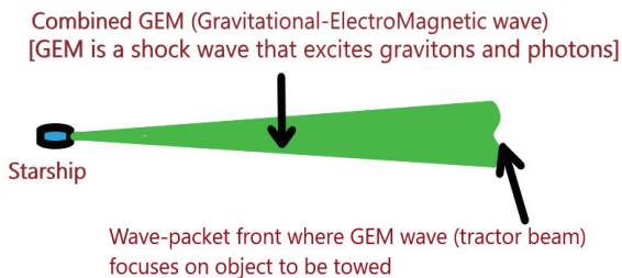
Figure 8: STARSHIP'S TRACTOR BEAM, PRODUCED FROM VECTOR-TENSOR-SCALAR GEOMETRY (there's a section about VTS Geometry earlier in this article)
