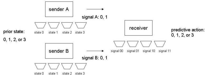
FIGURE 2. A more subtle sender-predictor game.
