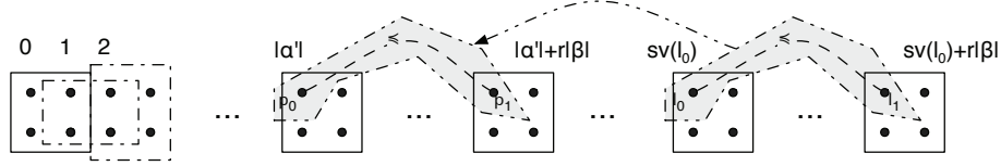
Figure 5: Example of translation by sv(l_0) - |\alpha'| .
