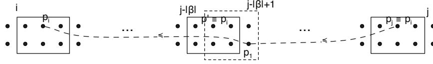
Figure 4: Relations between symbolic valuations i and j .
