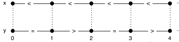
Figure 9: A weak symbolic model for Formula (6).
