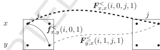
Figure 7: Definition of \mathbf{F}^< by local relations \mathbf{f}^< .
