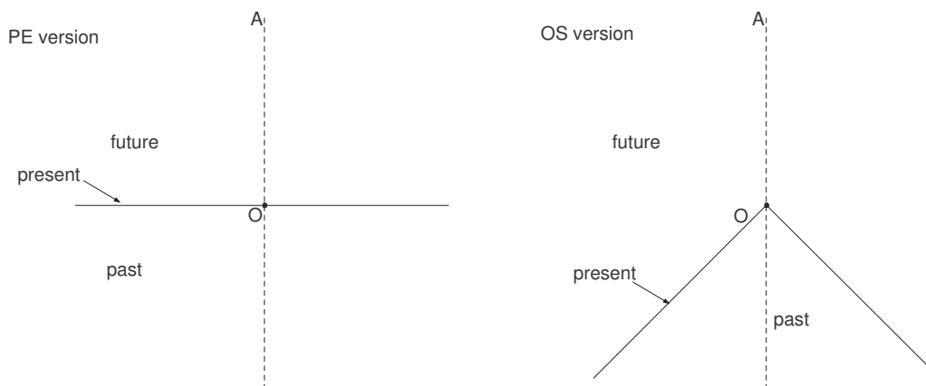
Figure 4: Representations of the past, present and future at O of an observer \mathcal{A} , according to PE and OS, respectively.
