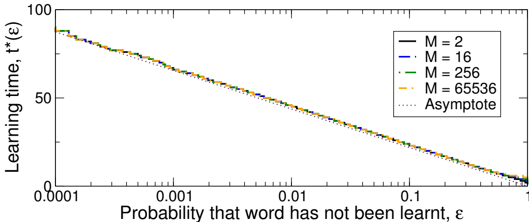
Figure 5: Time to learn a word with probability 1 - \epsilon with confounder frequencies governed by a logarithm a_n = c \frac{\ln(2)}{\ln(n+1)} , with c = 0.9 . Here the data for different sizes of the space of confounders, M , are indistinguishable except very close to \epsilon = 1 . The learning times are close to the asymptotic result t^*(\epsilon) \sim \ln(\epsilon)/\ln(c) even though formally in the limit M \rightarrow \infty the learning time diverges for all \epsilon .
