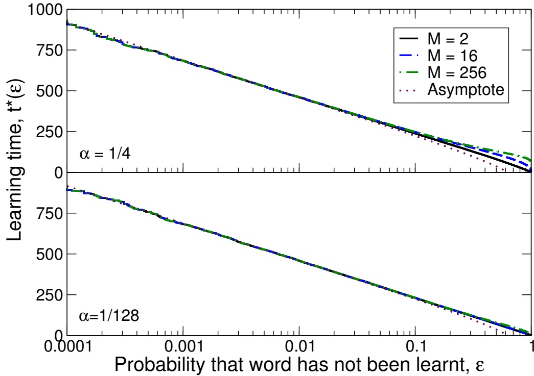
Figure 3: Time to learn a word with probability 1 - \epsilon with confounder frequencies governed by the power-law with c = 0.99 and \gamma = 0.01 . Meanings are correlated so that strings of neighbouring meanings are likely to appear, the degree of correlation being determined by \alpha . As in Fig. 2, learning time is independent of the number of incidental meanings, M . Furthermore, learning time is largely unaffected by correlations between meanings, as can be seen by comparing the upper and lower panels of this figure (within-episode correlations are substantially stronger in the lower panel), and indeed by comparing this figure to Fig. 2 (where there are no within-episode correlations): any differences from the uncorrelated case (Fig. 2) are confined to the large- \epsilon regime.
