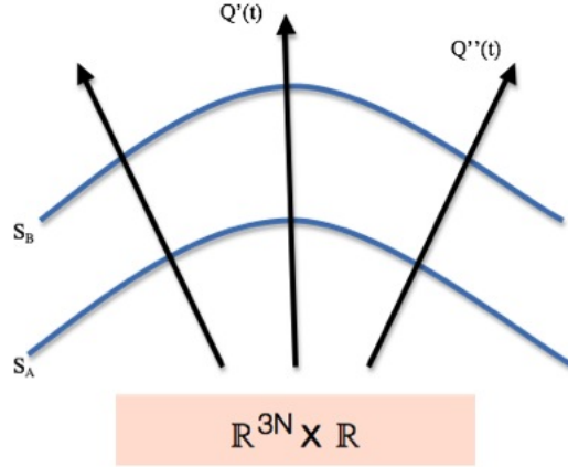
Figure 5.1: Hamilton-Jacobi theory
