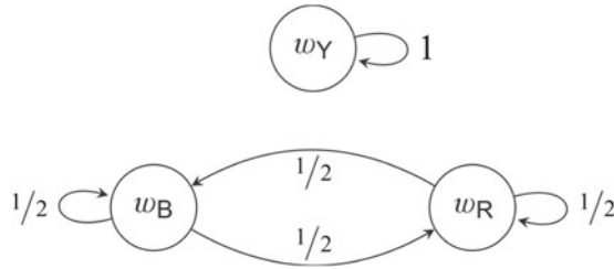
Fig. 1. Example of a probabilistic modal structure.
