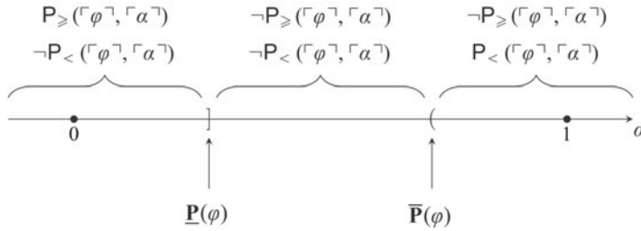
Fig. 5. Definition of \underline{P}(\varphi) and \overline{P}(\varphi) .
