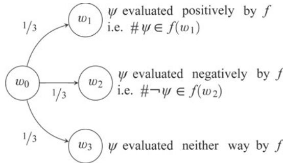
Fig. 2. A fragment of a probabilistic modal structure representing the information required to evaluate P_{\geq}(\ulcorner \psi \urcorner, \ulcorner \alpha \urcorner) in \Theta(f)(w_0) .
