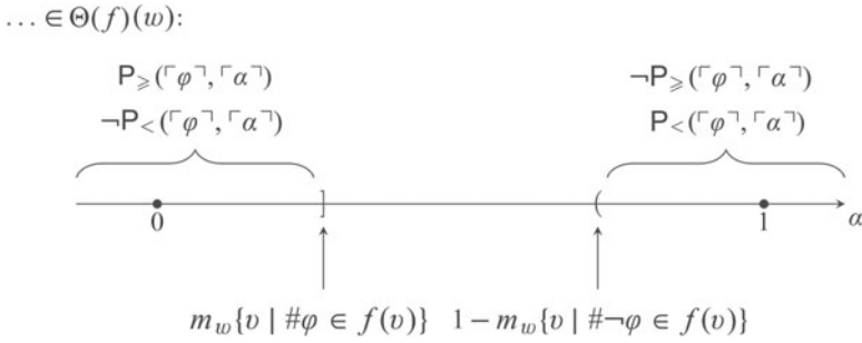
Fig. 3. How \Theta(f)(w) evaluates the probability of \varphi .
