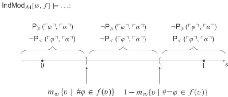
Fig. 4. How \text{IndMod}_{\mathcal{M}}[w, f] evaluates the probability of \varphi .
