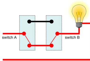
Fig. 3 Pretest I. Switch A and B are both down, and the light is on
