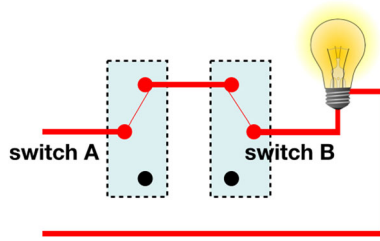
Fig. 4 Post-hoc test I. There is no wire between the two “down” positions
