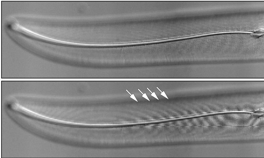
Fig. 5 Moiré . The top image is of a portion of a diatom acquired using a Zeiss LSM 510 confocal microscope in differential interference contrast mode. The bottom image is a demonstration image of the kind of moiré artifact that can occur in images that have repeating structures and have been incorrectly down-sampled or were initially undersampled . Note the curved artifacts ( arrows ) in the diatom in the bottom image. This artifact is the result of aliasing the periodic features in the diatom. This is a somewhat extreme example; however, users need to be aware that down-sampling an image (i.e., reducing the total number of pixels in X and Y) can reduce the information content of an image, and may introduce unwanted, and unnoticed, artifacts. Noise was removed from the top image using Photoshop CS2's despeckle filter and a conservative contrast stretch performed to enhance the image. The bottom image is a screen capture taken when the above image was viewed at 33% on screen and then the captured image was enlarged using the Photoshop CS3 nearest neighbor algorithm
