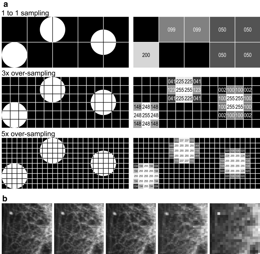
Fig. 3 a Sampling —theoretical. This illustration shows three bright (intensity = 255) spots that are aligned in different ways with the pixels on a sensor. Each spot is the same size; in each row the detectors are sampling the spot at higher frequencies. The left-most spot can be accurately measured at all three sampling levels. The other two spots give widely varying measurements that are more accurate as the sampling level increases. At 10× oversampling (not shown), all three spots measure exactly 10 pixels in both the x and y axes. In this example, it is assumed that there is no space between the pixels, though in reality this is never the case. In places where the spot did not fill the pixel, the mean intensity was measured using ImageJ (Rasband 1997–2009). This is similar to how a CCD camera treats a partially-illuminated pixel. These reduced-intensity pixels demonstrate how a feature is displayed using aliasing . If a user is too aggressive when processing an image, the aliased pixels can become bright enough to look like a real feature. This would be particularly problematic in the 1 to 1 sampling image, since the three spots could be blended together by over-processing, thus leading to a possible misinterpretation of the data. Note, this example assumes maximum brightness in every portion of the spot. In reduced light conditions (e.g., fluorescence microscopy), these assumptions may not be correct. b Sampling —example. A small area from the same field of view as that used in Fig. 4 was imaged on a Zeiss LSM 510 confocal microscope at 2048 × 2048 pixels, 1024 × 1024, 512 × 512, 256 × 256 and 128 × 128 pixels using the same optical magnification. The areas have been enlarged using the Photoshop CS3 nearest neighbor algorithm and each image was individually contrast stretched and a gamma adjustment of 1.1 was applied to clearly show the pixelation
