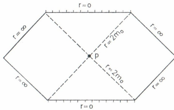
Figure 3.1: Carter-Penrose diagram of Schwarzschild spacetime. Each point in the diagram represents a 2-sphere in the spacetime manifold. (This diagram is taken from Geroch 1969 , with the author's permission.)
