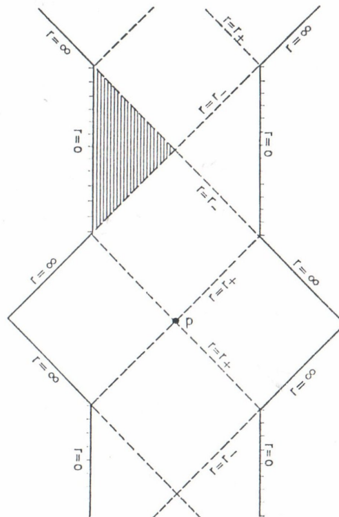
Figure 3.2: Carter-Penrose diagram of Reissner-Nordström spacetime. Each point in the diagram represents a 2-sphere in the spacetime manifold. (This diagram is taken from Geroch 1969 , with the author's permission.)
