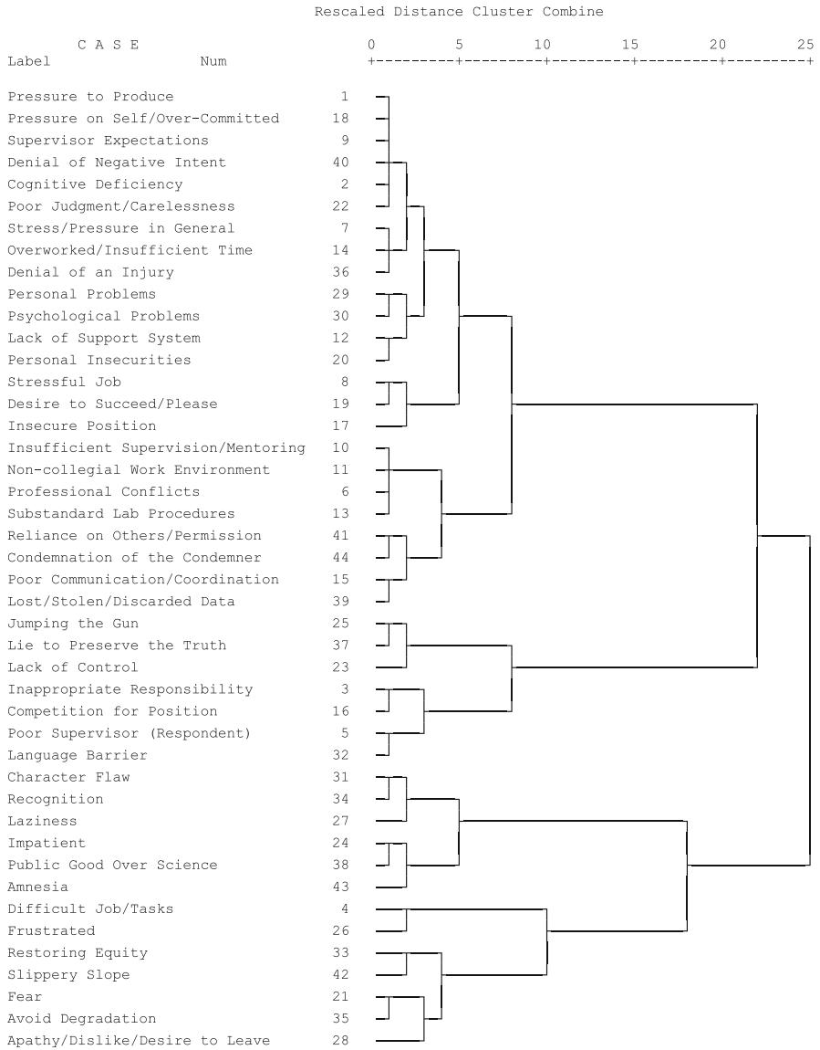
Fig. 2 Dendrogram of the 44 concepts
