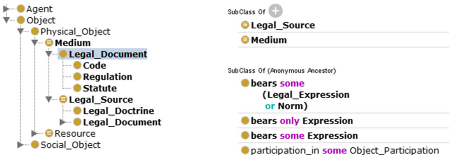
Fig. 3 Excerpt of the Core Module in Protégé
