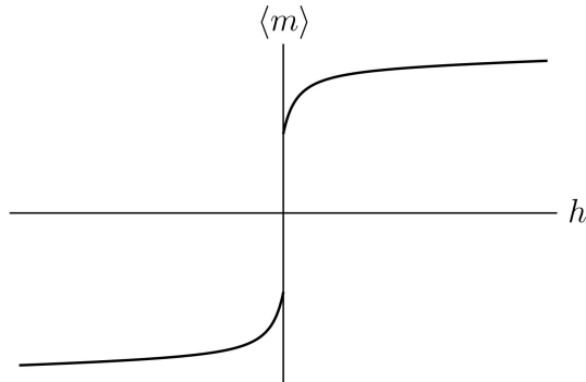
Figure 1: Sketch of the expected magnetisation as a function of the external magnetic field, h , for an Ising model on an infinite two dimensional lattice.
