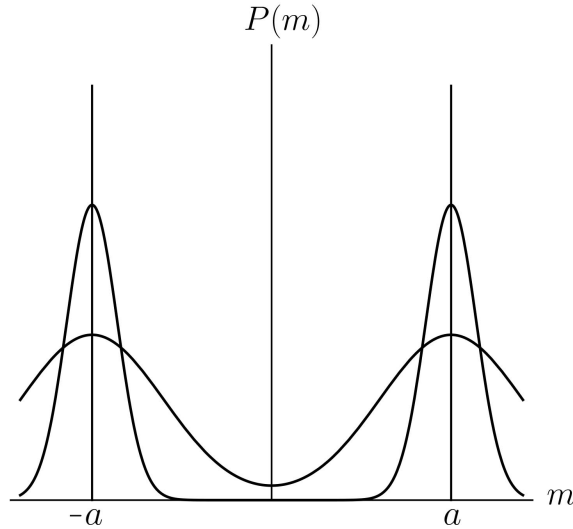
Figure 2: Sketch of P(m) below the critical temperature for an Ising model with small, large and infinite N .
