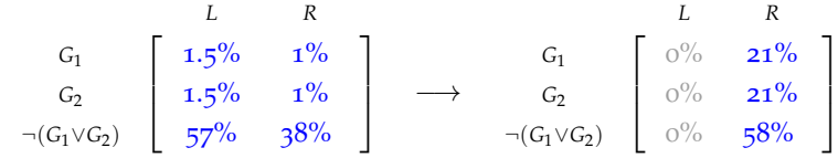
Figure 2: The right-hand-side distribution is the result of LP conditionalizing the left-hand-side distribution on the proposition R .
