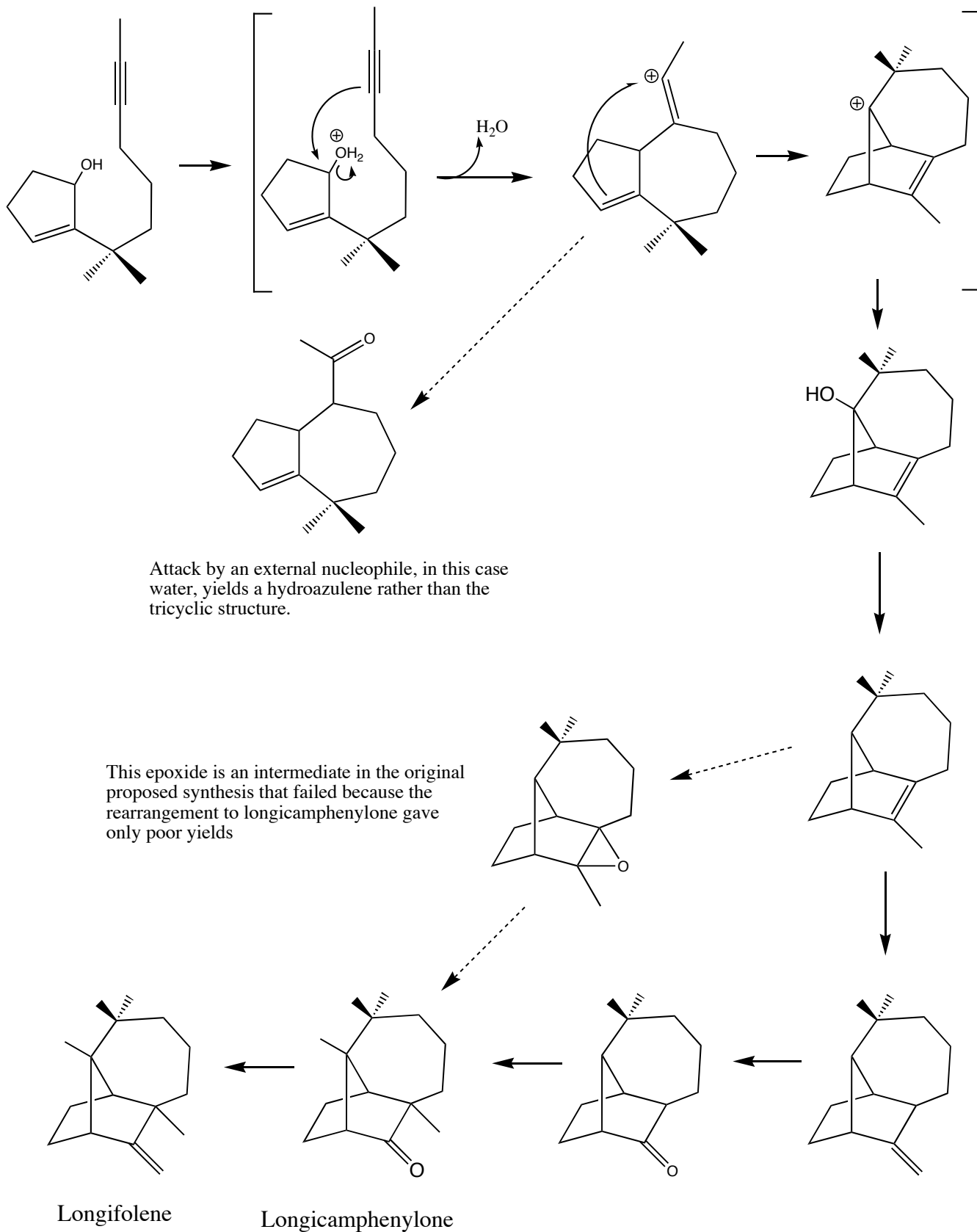
Figure 1: Sketch of a novel synthesis of Longifolene. A possible mechanism for the crucial step, with important side product indicated by the dashed line, is in brackets. An alternative, shorter route that failed in the lab is also indicated with dashed lines.
