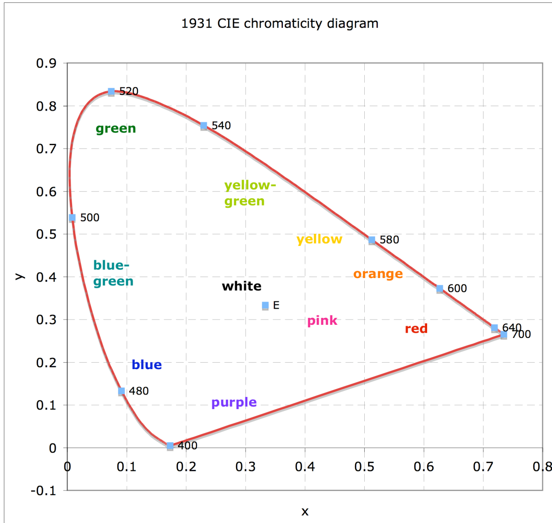
figure 1: 1931 CIE chromaticity diagram
