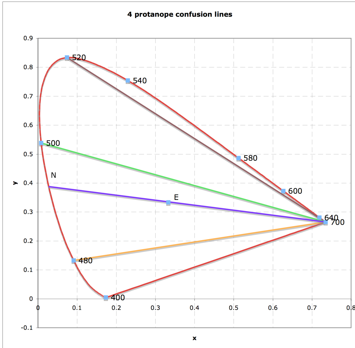
figure 2: 4 protanope confusion lines
