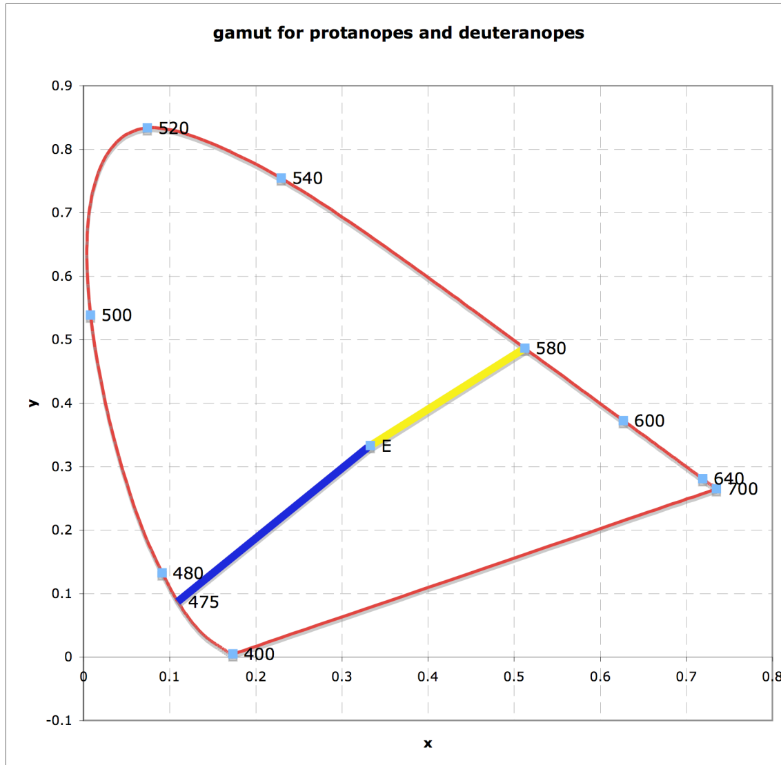
figure 3: gamut for protanopes and deuteranopes (on Standard Reduction View)
