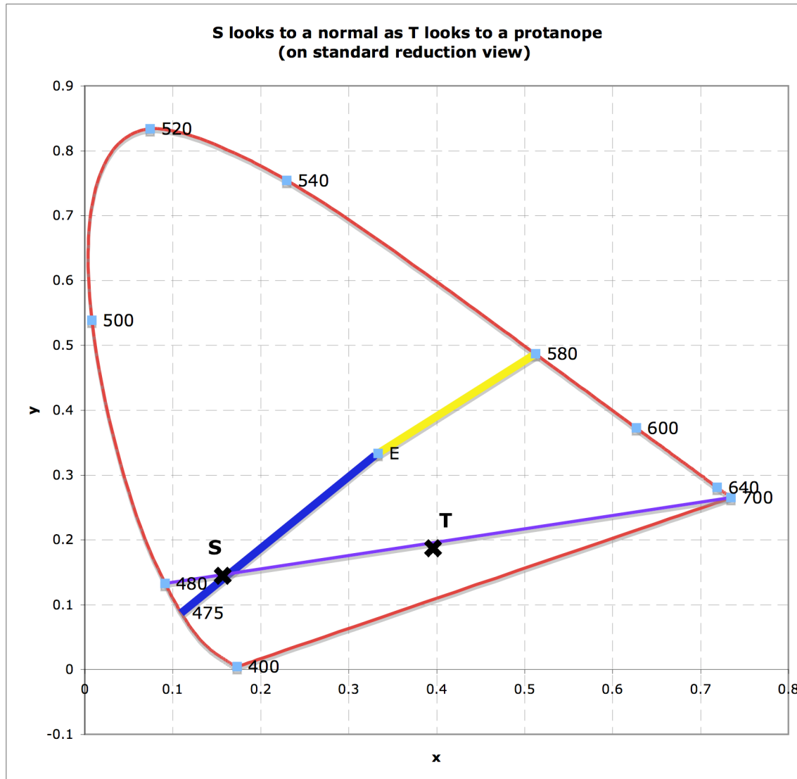
figure 4: S looks to a normal as T looks to a protanope
