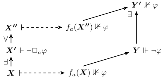
Fig. 1. f-refinability as used in the proof of Lemma 2.3.2, assuming \mathcal{M}, \mathbf{X} \not\Vdash \Box_a \varphi . Solid arrows are for the refinement relation \geq and dashed are for the function f_a .
