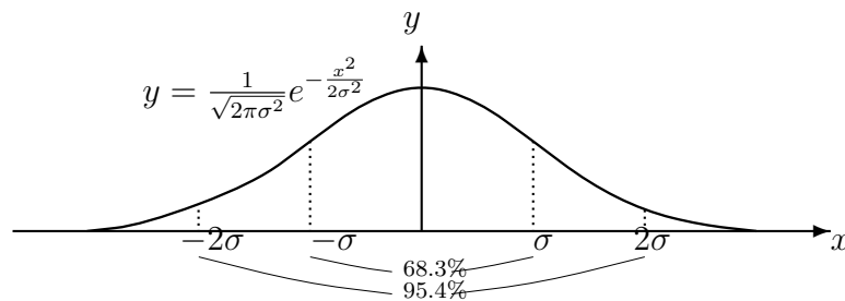
Figure 5.2: Error function
