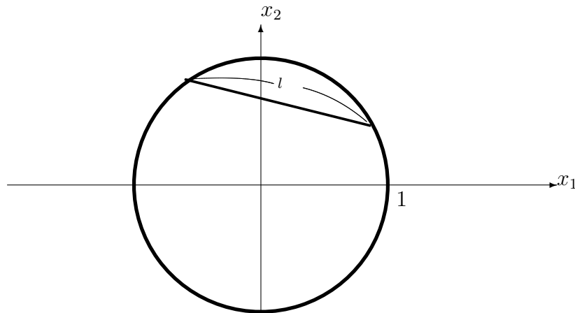
Figure 9.8: Bertrand's paradox
