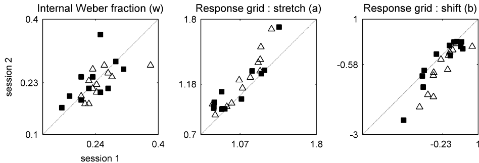
Fig. 8. Evolution of the internal Weber fraction ( w , left panel), and the two parameters of the affine transformation applied to the response grid (stretch on the middle panel and shift on the right panel) between the two experimental sessions in Experiment 2. X -axes represent the value of these parameters for the first session, and Y -axes the values for the second session. Dotted lines indicate the equality diagonal (first session = second session). Each dot represents one participant: participants presented with a larger inducer in the second session are marked as filled squares, and participants presented with a smaller inducer in the second session are marked as unfilled triangles. Values indicated on the axes correspond to the means for the first and second sessions. The graphs illustrate how each subject possesses an idiosyncratic value of parameters w , a and b , which is reproducible across the two sessions, and also demonstrate that only the parameters a and b are affected by calibration.
