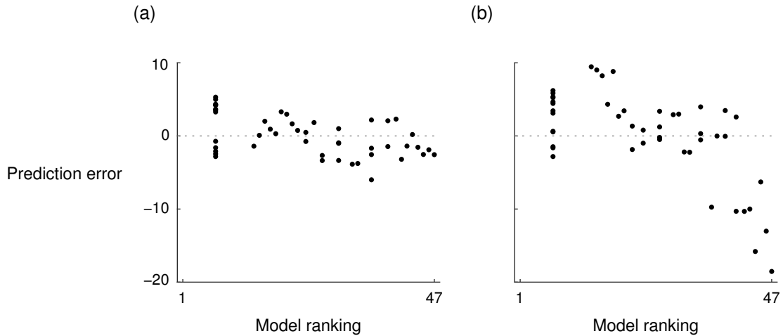
Figure 4. Residual plots for the inverse decision-making model predictions for (a) the positive-attributes and (b) negative-attributes conditions of Experiment 1.
