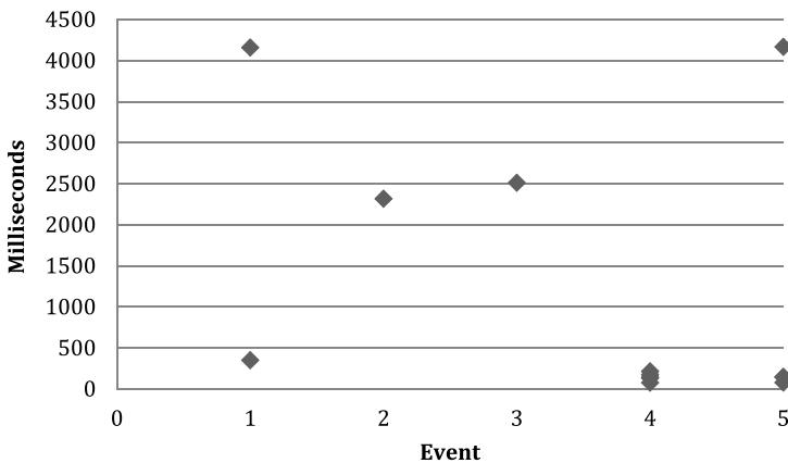
Fig. 4. Number of milliseconds for metric matches using the correlation algorithm within five events. We found a gradual improvement until an adequate match could not be found, at which point the retrieval times increased as the search space increased.
