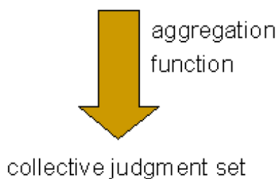
Figure 1: Judgment aggregation
