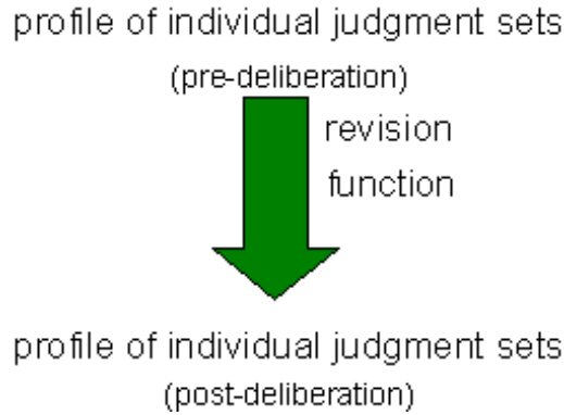
Figure 2: Judgment revision
