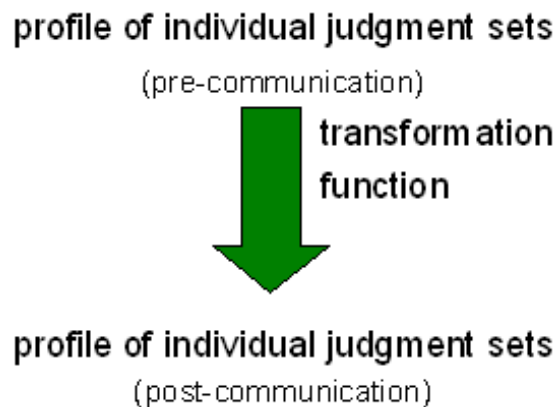
Figure 2: Judgment transformation
