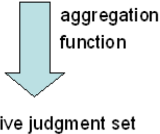
Figure 1: Judgment aggregation
