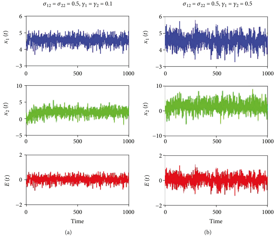
FIGURE 6: Parameter values for numerical simulations are given as follows: r_1 = 2, b_1 = 0.4, a_1 = 0.5, k = 6, q = 0.1, m_1 = 1, m_2 = 2, r_2 = 0.3, a_2 = 2, w = 5, c = 1, and v = 0.5 . Dynamical responses of system (3) with \sigma_{11} = 0.1, \sigma_{21} = 0.5, \sigma_{12} = 0.5, and \sigma_{22} = 0.5 and different values of \gamma_1 and \gamma_2 , where (a) \gamma_1 = \gamma_2 = 0.1 and (b) \gamma_1 = \gamma_2 = 0.5 .
