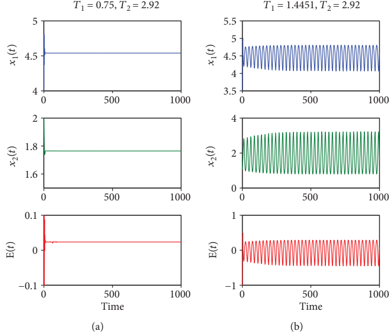
FIGURE 1: Parameter values are given as follows: r_1 = 2 , b_1 = 0.4 , a_1 = 0.5 , k = 6 , q = 0.1 , m_1 = 1 , m_2 = 2 , r_2 = 0.3 , a_2 = 2 , w = 5 , c = 1 , and v = 0.5 . When \sigma_{jk} = 0 ( j, k = 1, 2 ) and \gamma_i(u) = 0 ( i = 1, 2 ), dynamical responses of system (21) are plotted, where (a) \tau_1 = 0.75 , \tau_2 = 2.92 , and system (21) is locally asymptotically stable around (4.5384, 1.7647, 0.0231) and (b) \tau_1 = 1.4451 , \tau_2 = 2.92 , and system (21) is unstable stable around (4.5384, 1.7647, 0.0231) .
