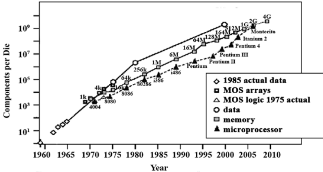
Figure 6 Moore's Law for integrated circuits, a logarithmic plot of Components per die from 1960 to 2010. Data and figure from (Moore, 2006); MOS is metal oxide semiconductor.
