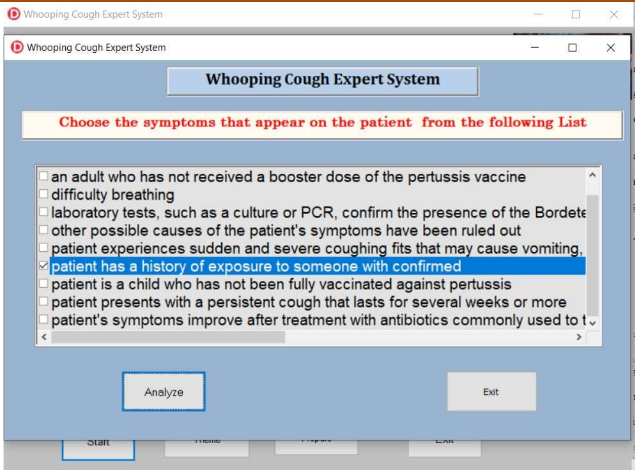
Figure 4: Inference Engine Implementation
