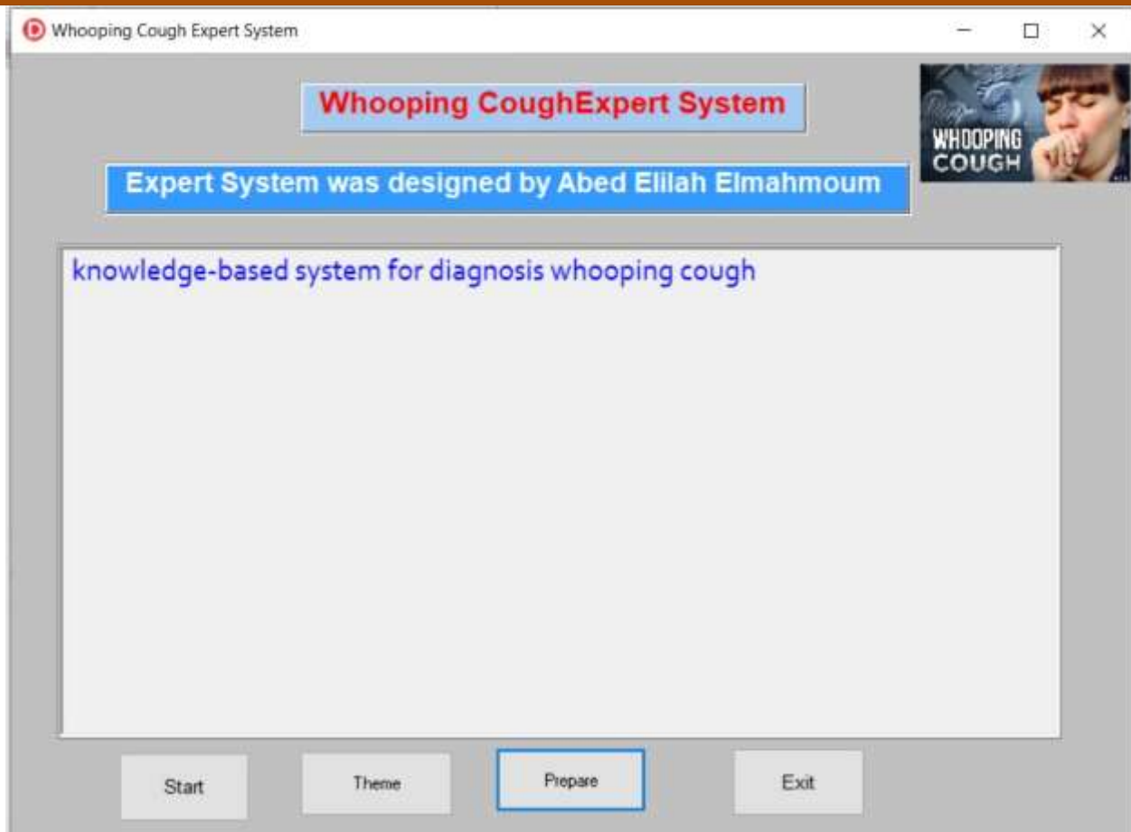
Figure 2: CLIPS Framework
