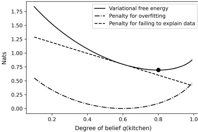
Fig. 2 Variational free energy F(p, q, x) as a function of the belief distribution q(w) when x = \text{meow} . The penalty for overfitting takes its minimum value when q(\text{kitchen}) = 0.6 = p(\text{kitchen}) . That is because choosing a posterior that is identical to the prior is the extreme opposite of overfitting. The penalty for failing to explain the data takes its minimum value when probability 1 is assigned to the cat being in the kitchen. That is because the kitchen is the best explanation for the cat's meowing. Variational free energy F takes its minimum value at 0.8 (solid black circle) between the minima of its two component costs. FREE ENERGY PRINCIPLE (INFERENCE) therefore counsels that q(\text{kitchen}) = 0.8 = \frac{4}{5} , in agreement with the solution given by BAYESIAN PRINCIPLE. The code to generate this graph can be found at https://github.com/stephenmann/fep
