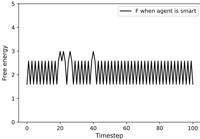
Fig. 5 Variational free energy over time for an agent that controls its external state in a survivable manner. The agent's control over its external state is 95% accurate; occasionally its grasp slips and free energy increases beyond the average. The code to generate this figure can be found at https://github.com/stephenfmann/fep
