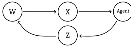
Fig. 3 The basic model of action. An agent can produce an act, z , in order to bring about states w that in turn produce outcomes x . Active inference employs a controversial dual interpretation of p(w) and p(x) as probability distributions and preference distributions over hidden states and sensory states respectively
