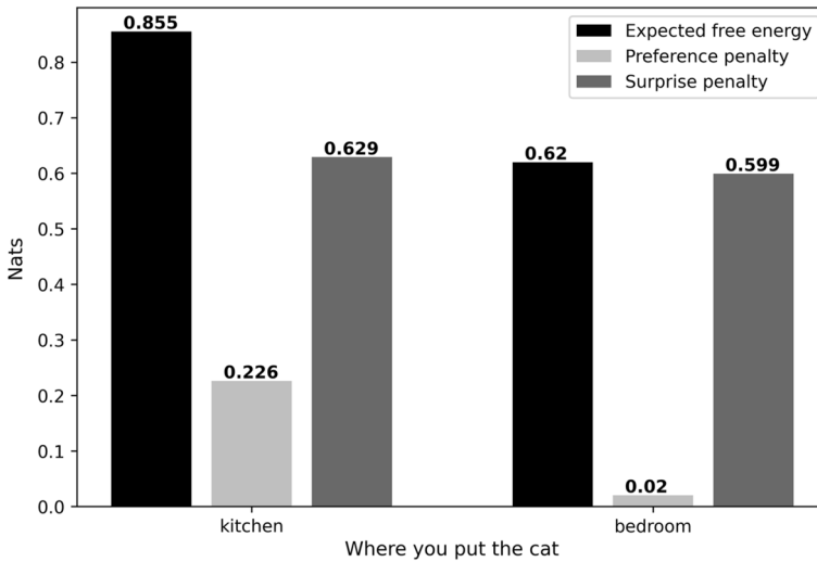
Fig. 4 Expected free energy G(p, q, z) when putting the cat in the kitchen or bedroom. The value of G is lowest when z = \text{bedroom} , so FREE ENERGY PRINCIPLE (ACTION) dictates that that is where you should put the cat. The surprise penalty for both acts is about the same, because in either case you cannot be very certain about whether the cat will be meowing or purring at the next time step. However, the preference penalty for putting the cat in the bedroom is relatively small, because q(w|\text{put cat in bedroom}) = \left(\frac{5}{10}, \frac{5}{10}\right) is relatively close to the distribution p(w) = \left(\frac{6}{10}, \frac{4}{10}\right) . Intuitively: if you want the cat to spend roughly equal time in both places, you shouldn't put it in the kitchen, because it will stay there. The code to generate this graph can be found at https://github.com/stephenfmann/fep
