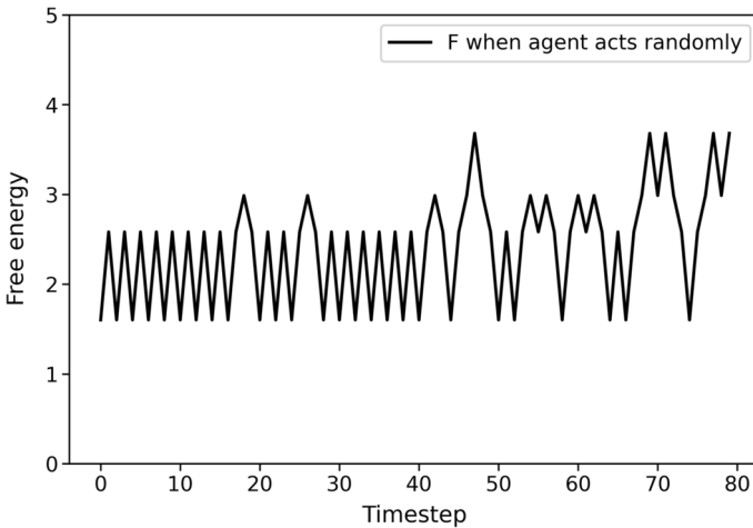
Fig. 6 Variational free energy over time for an agent that acts randomly. After 80 timesteps the agent dies and free energy takes an infinite value. The code to generate this figure can be found at https://github.com/stephenfmann/fep
