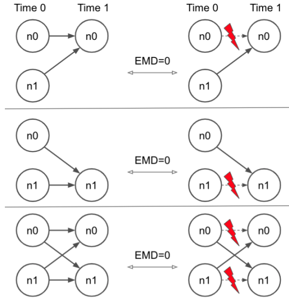
Figure 2: For candidate part \{n_0, n_1\} , each potential purview has a minimal disconnection that does not affect the future state of the system. Thus, \{n_0, n_1\} as a candidate part does not have any effect into the future of this system (zero effect).
