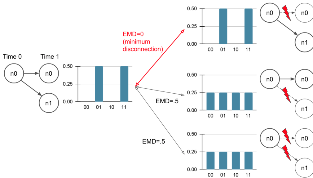
Figure 1: n_0 's future influence (effect). Among n_0 's potential candidate purviews, \{n_0, n_1\} has 0 influence as there is a minimal disconnection from n_0 to n_0 (top, right) that does not affect anything on the probability distribution of the system's state in the future.
