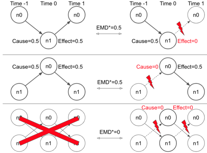
Figure 3: To assess the degree of the existence of a system, we compare the set of probability distributions for the original system (left) and the minimally unidirectionally disconnected system (right). Upon the disconnection, n1 has 0 effect and n0 has 0 cause, thus they do not exist. \{n0, n1\} also has minimal disconnection into its future and past purview making its effect and cause to be 0. Thus \{n0, n1\} also does not exist upon the disconnection. In sum, with a system-level minimal disconnection, nothing exists. The (generalized) earth mover's distance (EMD*) between the two distributions (left and right) arrives at a degree of integrated information of 1.
