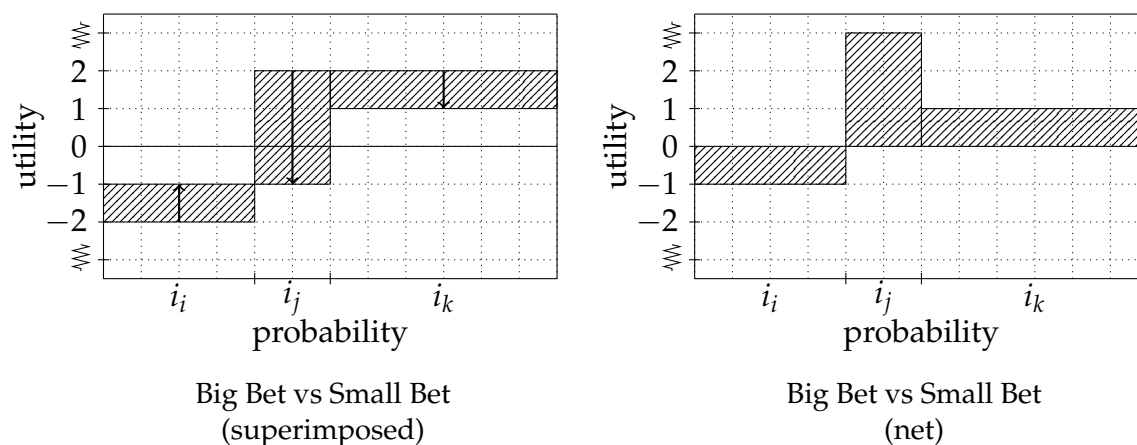
Figure 10: Big Bet vs Small Bet (difference minimizing)
