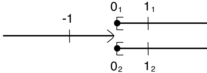
Figure 1: The branching real line as a simple non-Hausdorff space. A basis for the topology is given by the open intervals in both tracks, reaching into the common part on the left.
