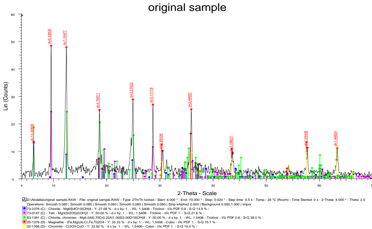
Figure 2. X-ray diffraction (XRD) pattern of chromite sample.
