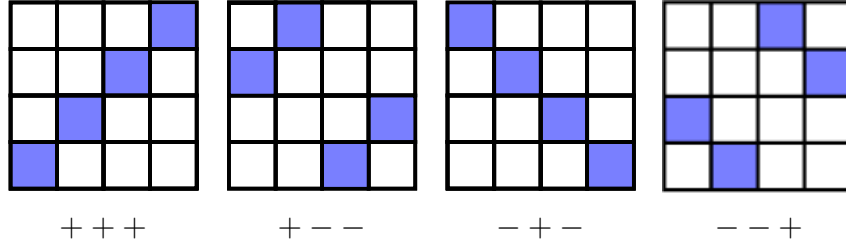
Figure 4: Common eigenstates of \sigma_x \otimes \sigma_x, \sigma_y \otimes \sigma_y, \sigma_z \otimes \sigma_z .
