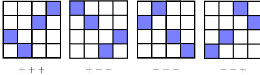
Figure 5: Common eigenstates of \sigma_x \otimes \sigma_y, \sigma_y \otimes \sigma_x, \sigma_z \otimes \sigma_z .
