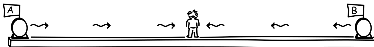
Figure 2. Einstein's definition of simultaneity
