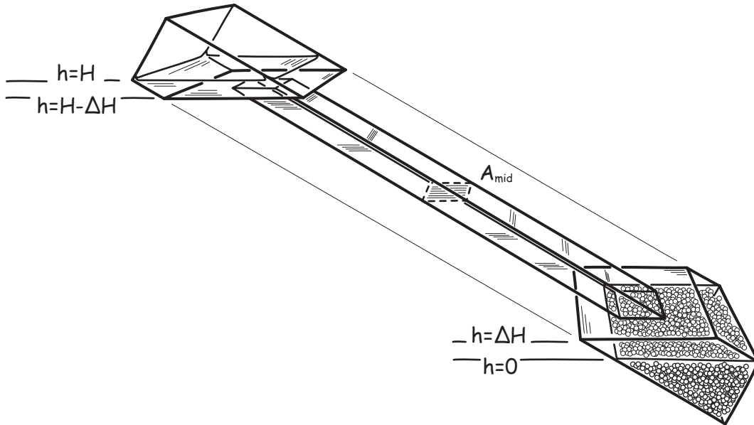
Figure 4. Dish with Spatial Volume of Intermediate States Reduced.
