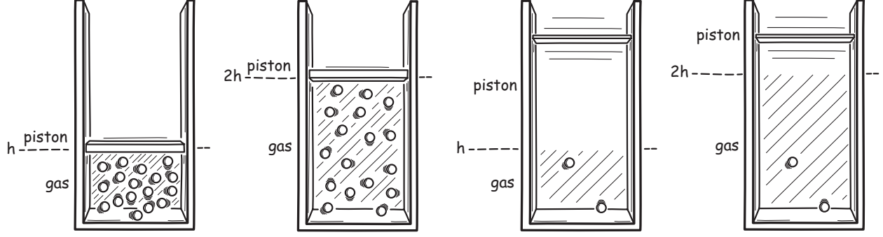
Figure 1. Microstates of h -states are Distinct only for Macroscopic Gases
