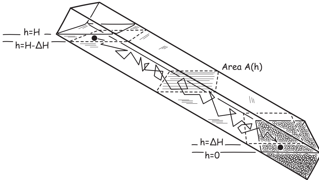
Figure 3. Gravity Suppresses Fluctuations in a Brownian Particle
