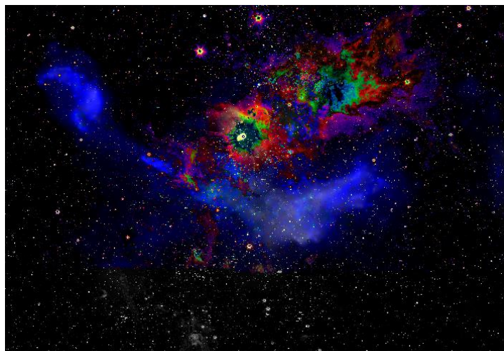
Fig. 8. Part of the dark matter cluster near black hole shadow made visible by multispectral quantum processing.
