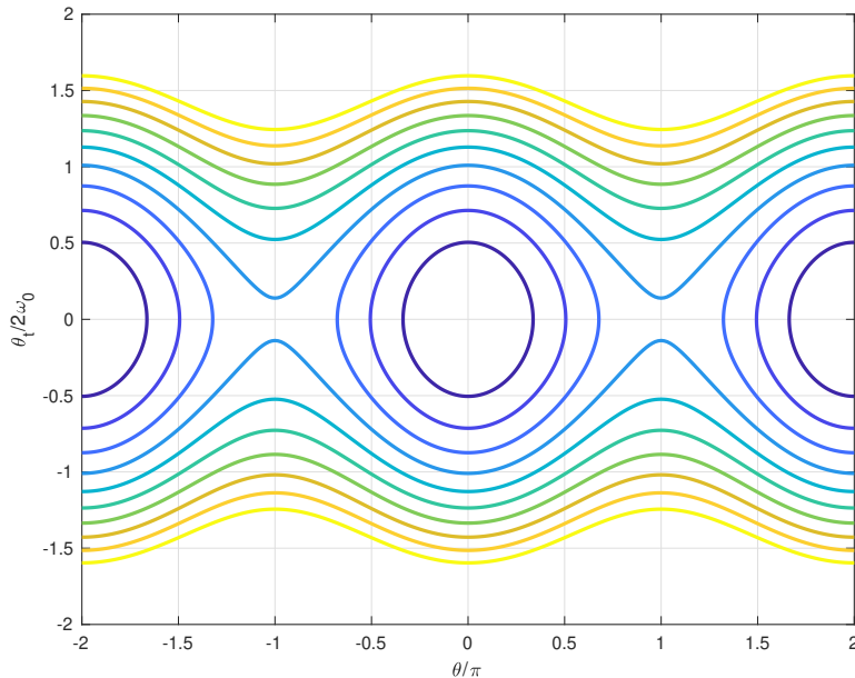
Figure 2: Motion of a simple pendulum for arbitrarily large oscillations (constant energy contours in phase space).
