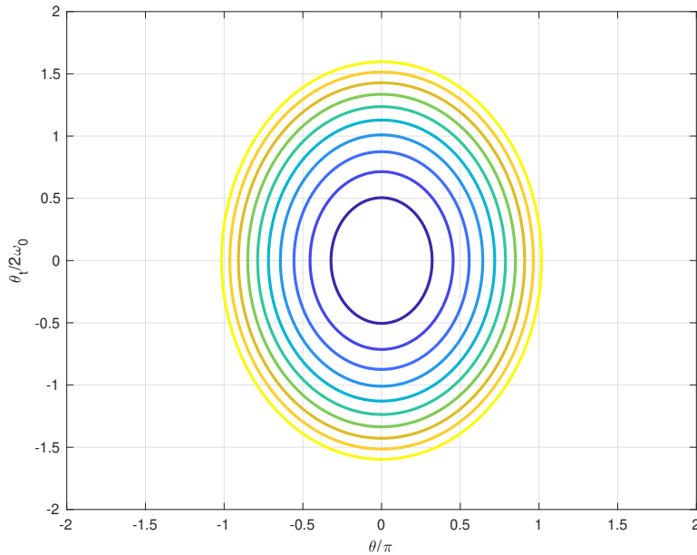
Figure 3: Motion of a simple pendulum for small oscillations (constant energy contours in phase space).
