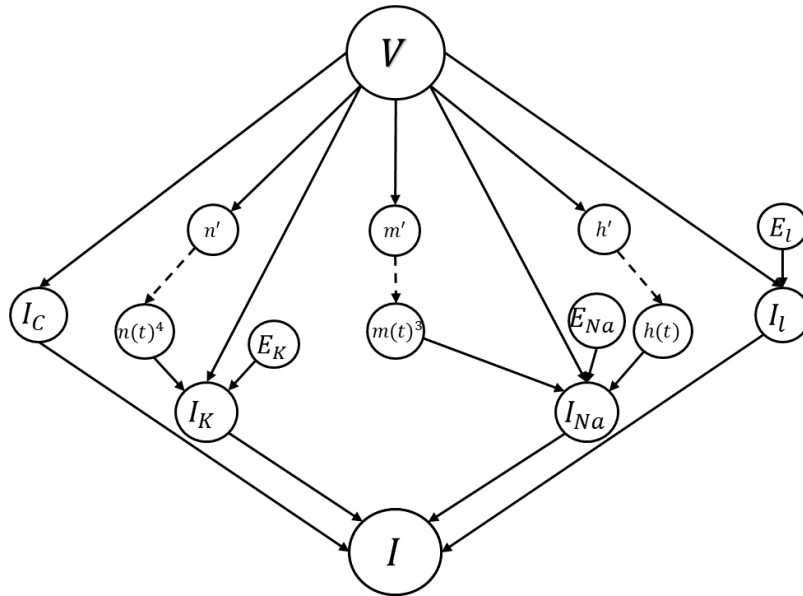
Figure 1. A graphical representation of functional relationships in the HH equations. Arrows reflect causal and constitutive relations between variables. V represents voltage, I 's represent the total and component currents, and E 's represent equilibrium voltages. Primed variables reflect the rate of change of the conductance terms m , n , and h . Terms not shown, such as the alphas and betas for sodium and potassium, are treated as parameters. Following Iwasaki and Simon (1994) and Voortman, Dash, and Druzdzel (2012), integration over time is represented with dashed lines. Consistent with their experimental practice, voltage is treated as an exogenous, experimenter-controlled variable. In simulating the action potential and related phenomena, V is no longer regarded as exogenous and is instead determined by integrating ionic currents (Hodgkin and Huxley's discussion of simulation procedures covers 522-40 in the paper).
