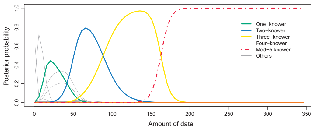
Fig. 6. Learning results for a Mod-5 system.
