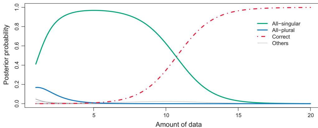
Fig. 5. Learning results for a singular/plural system.
