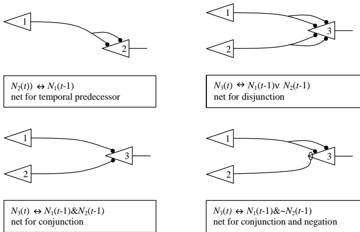
Figure 1. Diagrams of McCulloch and Pitts nets. In order to send an output pulse, each neuron must receive two excitory inputs and no inhibitory inputs. Lines ending in a dot represent excitory connections; lines ending in a hoop represent inhibitory connections.
