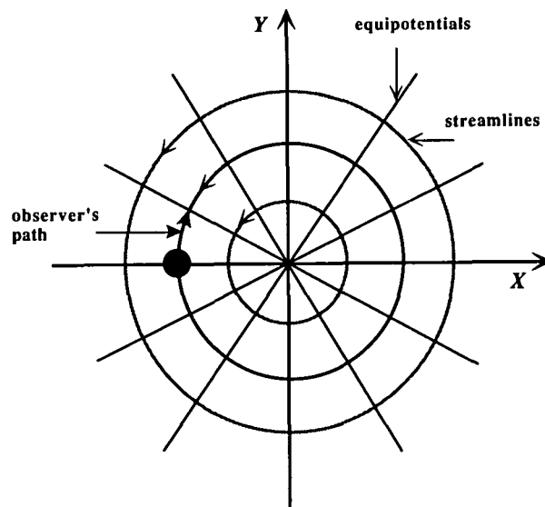
Figure 1 (Kim and Turvey). Circular flow field defined by the complex potential F(z) = K/(2\pi i)\ln z . The equipotential lines are the straight lines and the streamlines are the concentric circles. The flow circles around the origin, from which the observer's path lies with radius r .
