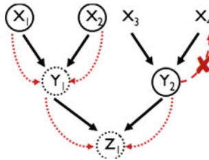
Fig. 3 Constructing fixed points on a dynamics
