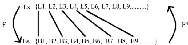
Figure 3. One-to-one and Into Function of mind-brain relationship.
