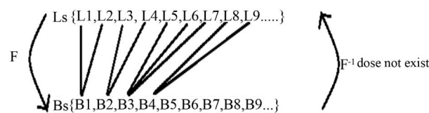
Figure 4. Many-to-one and onto function of mind-brain relationship.
