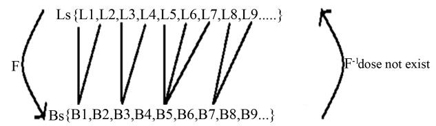
Figure 5. Many-to-one and into function of mind-brain relationship.
