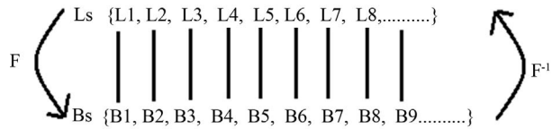
Figure 2. One-to-one and onto function of mind-brain relationship.
