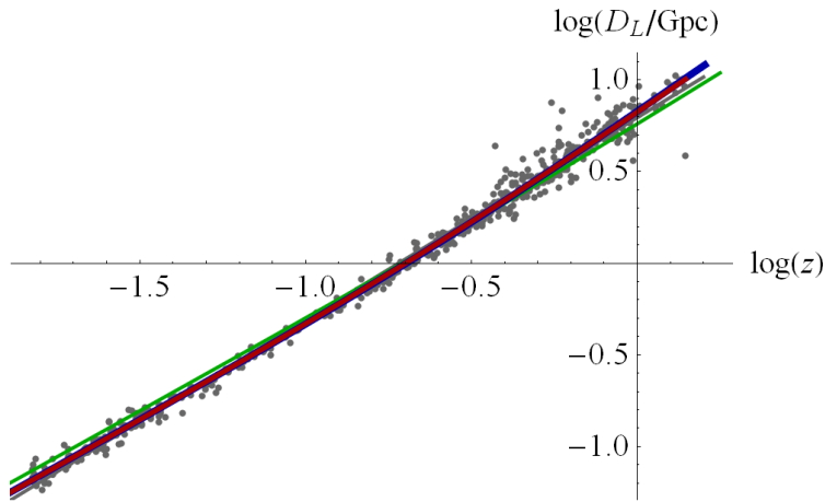
Fig. 6 Plot of transformed Union2 data along with the best fits for linear regression (gray), EdS (green), \Lambda CDM (blue), and MORC (red).
