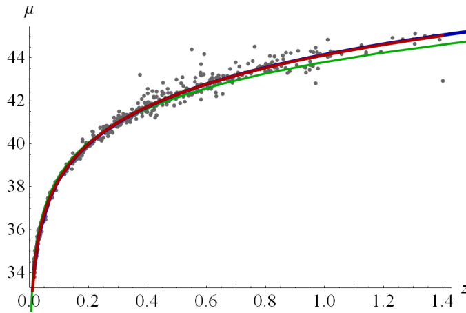
Fig. 7 Plot of Union2 data along with the best fits for EdS (green), \Lambda CDM (blue), and MORC (red). The MORC curve is terminated at z = 1.4 in this figure so that the \Lambda CDM curve is visible.
