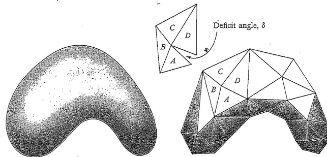
Figure 42.1. A 2-geometry with continuously varying curvature can be approximated arbitrarily closely by a polyhedron built of triangles, provided only that the number of triangles is made sufficiently great and the size of each sufficiently small. The geometry in each triangle is Euclidean. The curvature of the surface shows up in the amount of deficit angle at each vertex (portion ABCD of polyhedron laid out above on a flat surface).
