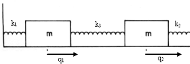
Fig. 4 Coupled harmonic oscillators.
