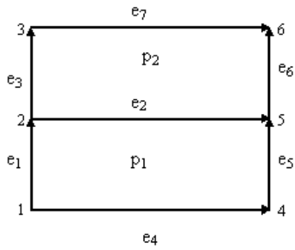
Fig. 3 Graph with six vertices, seven links e_i and two plaquettes p_i .
