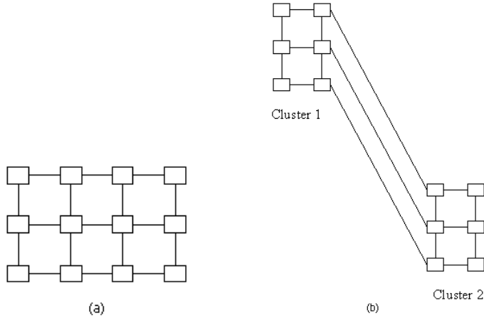
Fig. 1 (a) Topological Graph - This spacetime matter graph depicts four sources, i.e., the columns of squares. The graph's actional \mathbf{K}/2 + \mathbf{J} , such that \mathbf{K} \cdot \mathbf{v} \propto \mathbf{J} , characterizes the graphical topology, which underwrites a partition function Z for spatiotemporal geometries over the graph. (b) Geometric Graph - The topological graph of (a) is endowed with a particular distribution of spatiotemporal geometric relations, i.e., link lengths as determined by the field values Q . Clusters 1 & 2 are the result of this geometric process for a particular distribution of field values Q .
