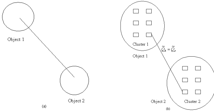
Fig. 2 (a) Classical Physics - Classical Objects result when the most probable field values \mathbf{Q}_0 yield spatiotemporally localized Clusters 1 & 2 as in Figure 1b. The lone link in this figure represents the average of the link lengths obtained via the most probable field values \mathbf{Q}_0 . The most probable values \mathbf{Q}_0 are found via \mathbf{K} \cdot \mathbf{Q}_0 = \mathbf{J} , so this is the origin of classical physics. (b) Quantum Physics - A particular outcome \tilde{Q}_0 of a quantum physics experiment allows one to compute the k^{\text{th}} link length of the geometric graph in the context of the classical Objects comprising the experiment, e.g., Source, beam splitters, mirrors, and detectors. The partition function provides the probability of this particular outcome, i.e., P(\tilde{Q}_k = \tilde{Q}_0) = \frac{Z(\tilde{Q}_k = \tilde{Q}_0)}{Z} .
